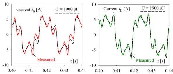
Figure 4: Measured and calculated no-load line currents at C = 1900 pF
