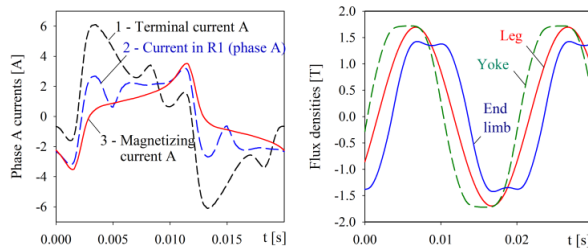
Figure 5: Phase currents (left) and flux densities (right) of the 5-legged unit
