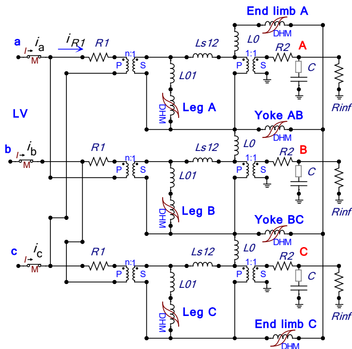
Figure 2: ATPDraw model of 786 MVA, YNd11 transformer
