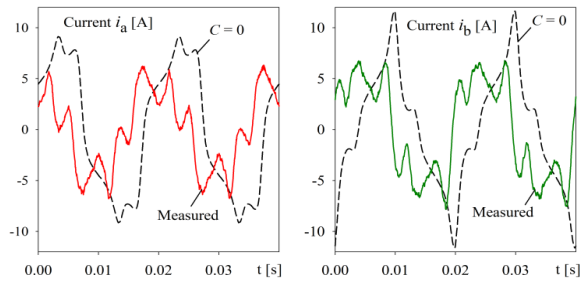
Figure 3; Measured and calculated no-load line currents at C=0
