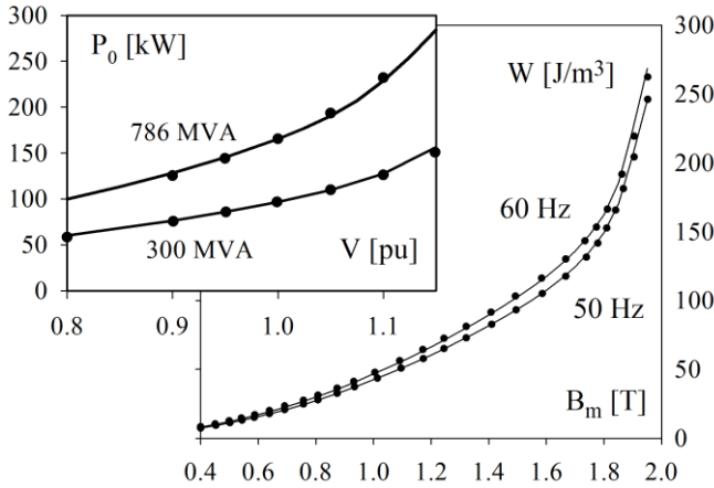
Figure 1: Specific losses W of the steel and no-load transformer losses P_0
