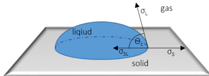
Figure 2.3: Contact Angle at a solid-liquid-gas contact line [25].
